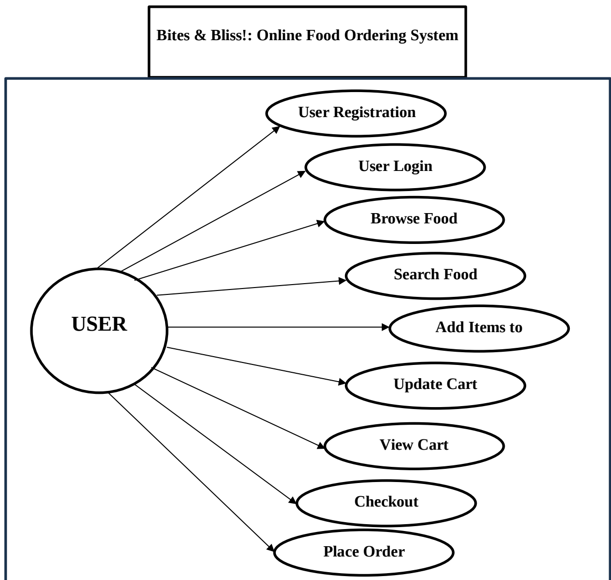
Fig. 2.1: Use Case Diagram of Bites & Bliss! Online Food Ordering System
