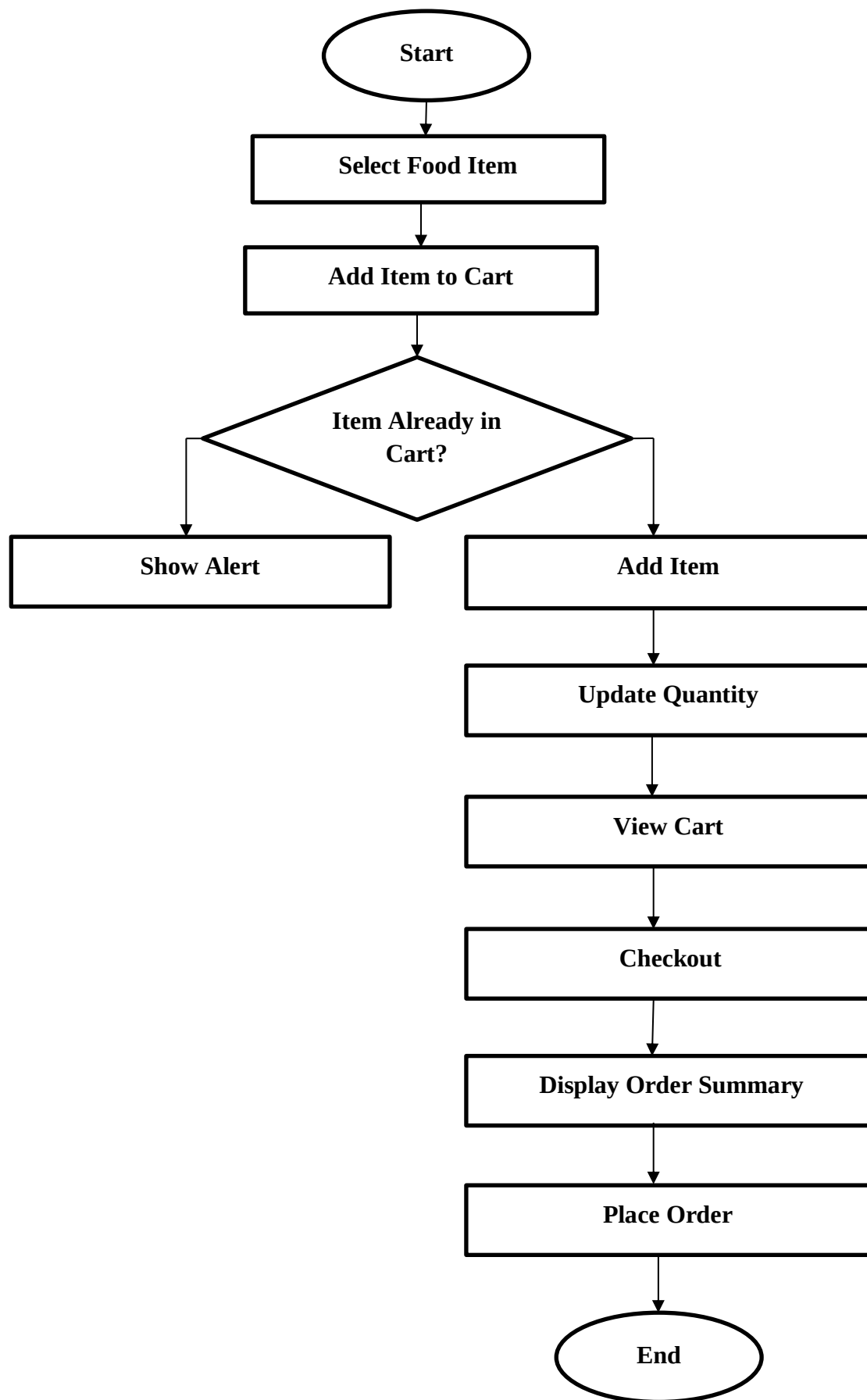
Fig. 2.2: Functional Flow of Cart and Checkout Process
